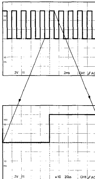
Figure 5-8 Magnified Waveform
