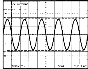
Figure 5-19: Cursor Measurement
