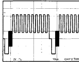
Figure 5-14(b) TV-H
