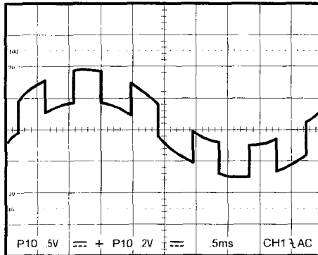
Figure 5-6 Typical ADD waveform
